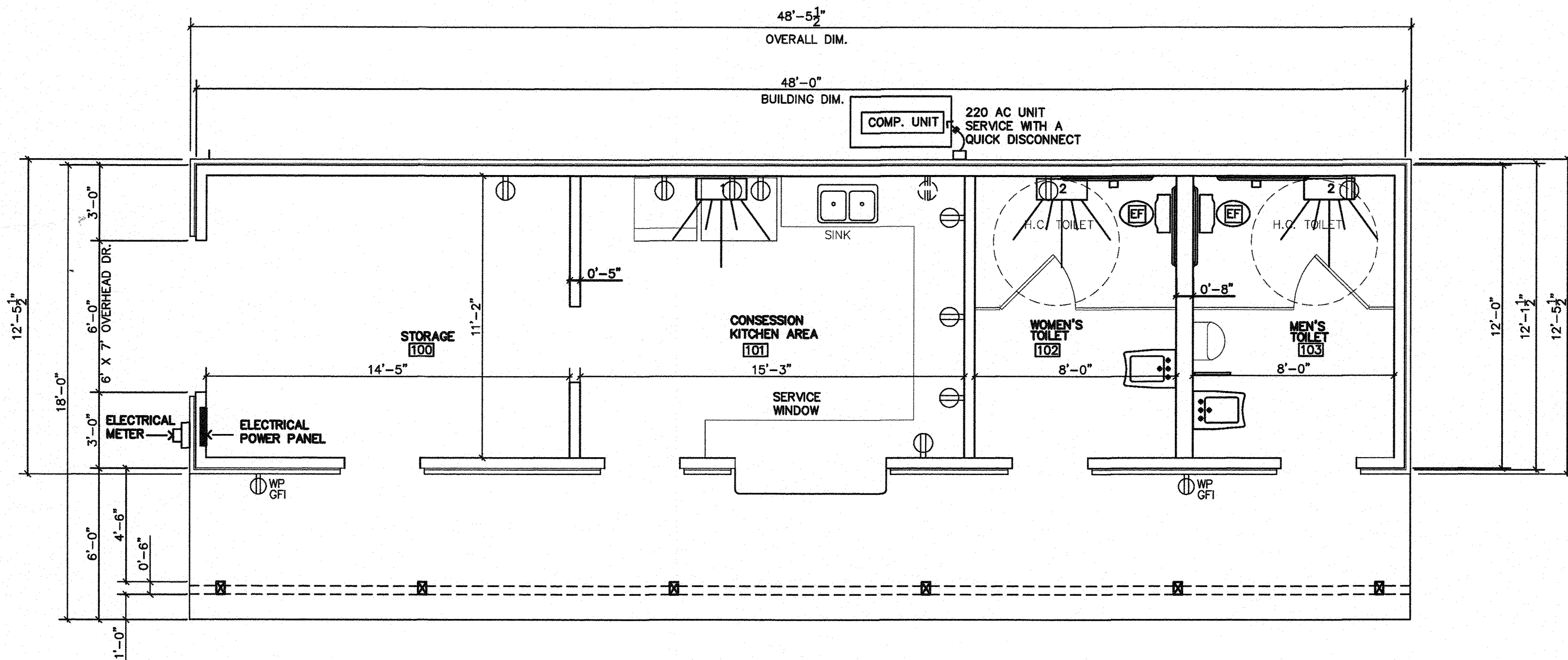
UNKNOWN A ELECTRICAL POWER PLAN SCALE: 1/4" = 1'-0"
