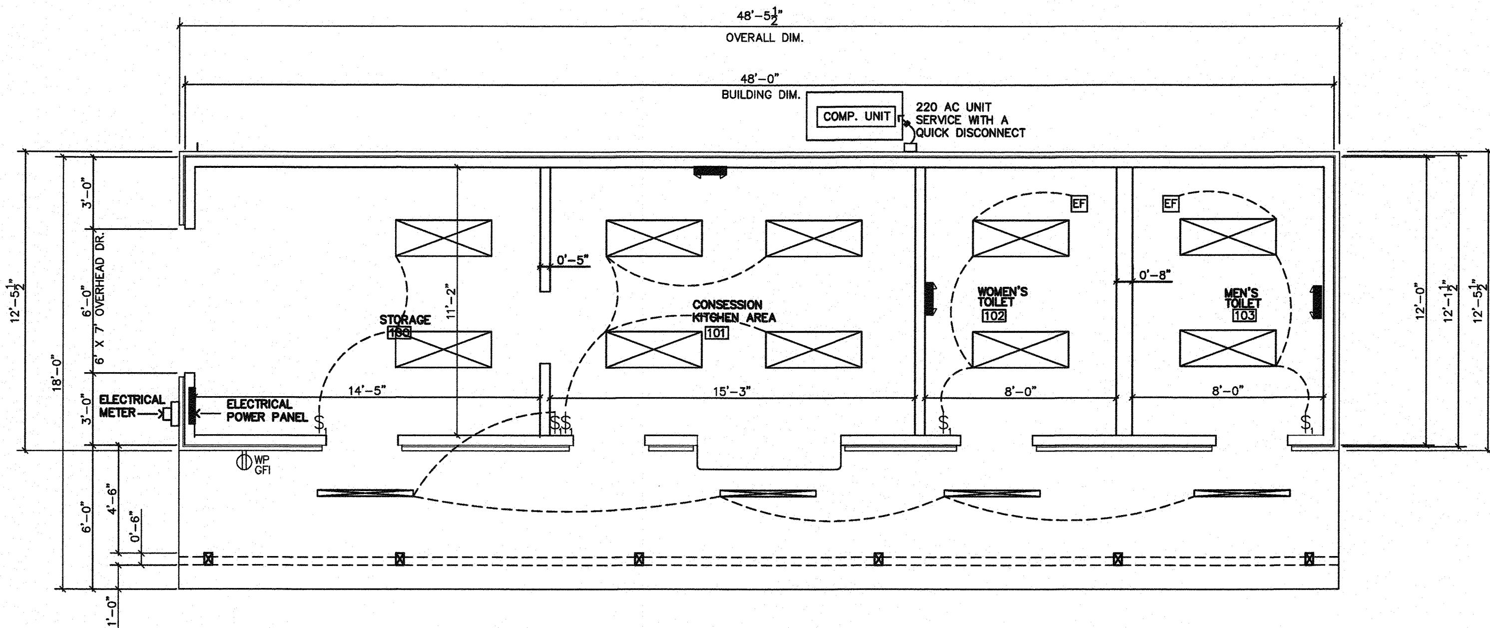
UNKNOWN A ELECTRICAL LIGHTING PLAN SCALE: 1/4" = 1'-0"
