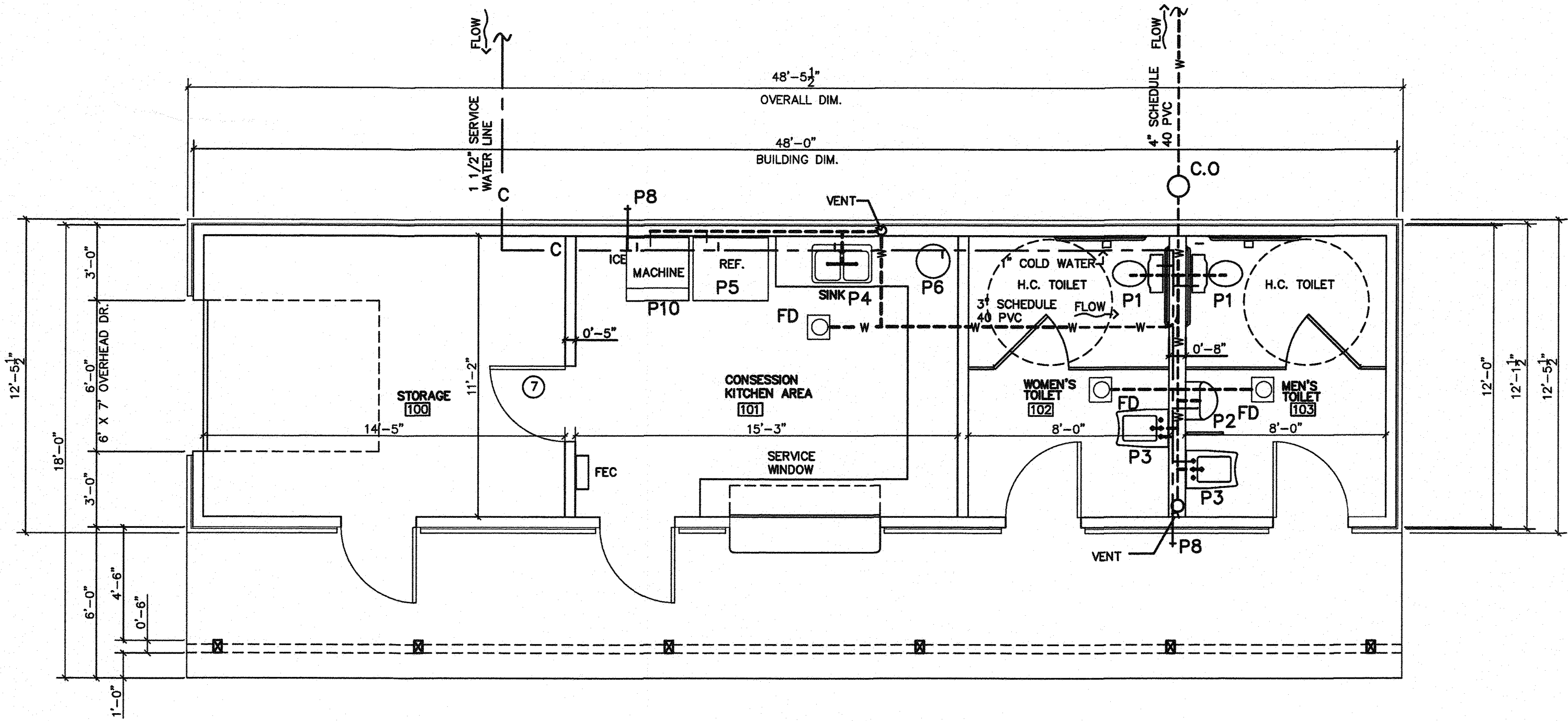
A PLUMBING PLAN P100P100 SCALE: 1/4" = 1'-0"
